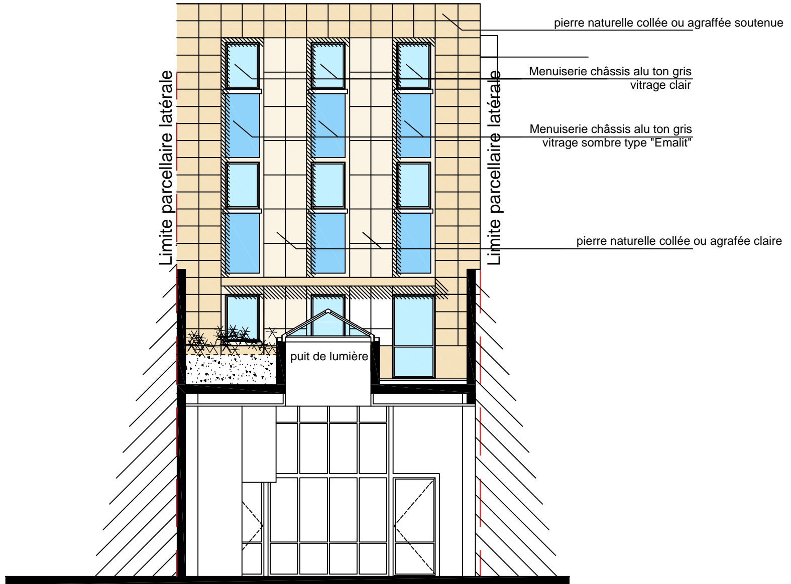
COUPE FACADE BB
